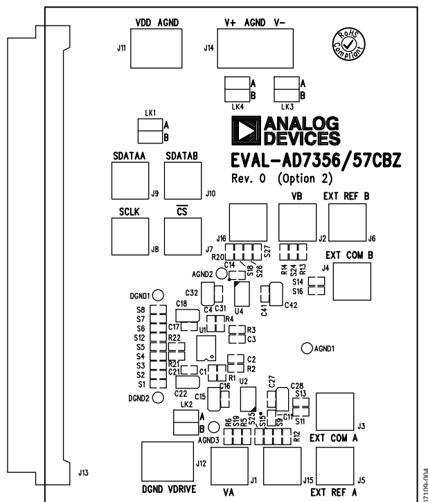
Figure 5. Silkscreen Top
