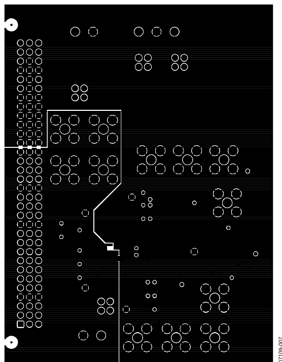
Figure 8. Layer 2 Artwork, Ground Planes
