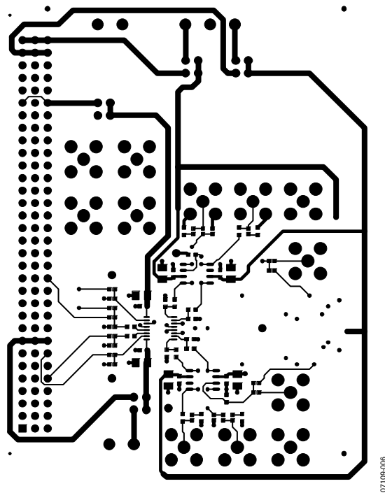
Figure 7. Layer 1 Artwork, Top
