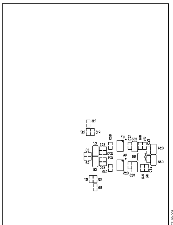
Figure 6. Silkscreen Bottom
