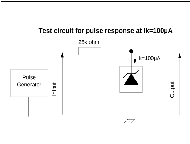
Figure 7. Test circuit for pulse response at I_k=100\mu A
