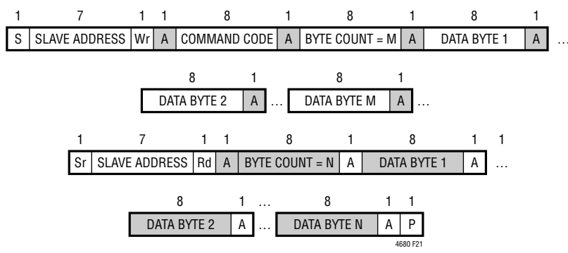
Figure 21. Block Write – Block Read Process Call
