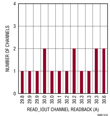
READ_IOUT of 16 LTM4680 Channels 12\text{V}_{\text{IN}} , 1\text{V}_{\text{OUT}} , T_J = 25^{\circ}\text{C} , I_{\text{OUT}n} = 30\text{A} , System Having Reached Thermally Steady-State Condition, No Airflow
