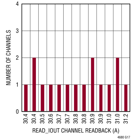
READ_IOUT of 16 LTM4680 Channels 12\text{V}_{\text{IN}} , 1\text{V}_{\text{OUT}} , T_J = -40^{\circ}\text{C} , I_{\text{OUT}n} = 30\text{A} , System Having Reached Thermally Steady-State Condition, No Airflow
