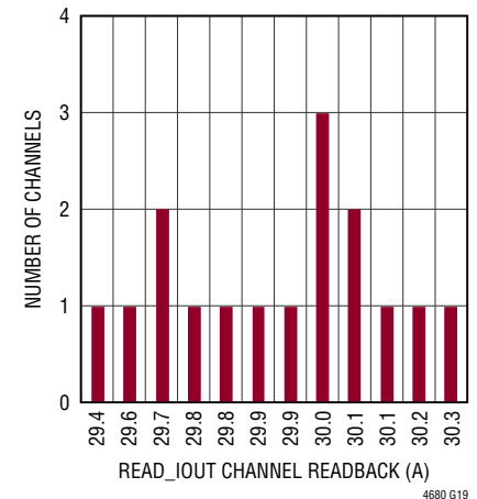
READ_IOUT of 16 LTM4680 Channels 12\text{V}_{\text{IN}} , 1\text{V}_{\text{OUT}} , T_J = 125^{\circ}\text{C} , I_{\text{OUT}n} = 30\text{A} , System Having Reached Thermally Steady-State Condition, No Airflow
