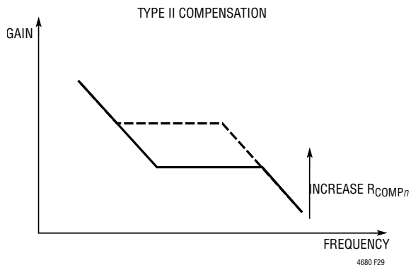
Figure 29. R_{COMP} Adjust
