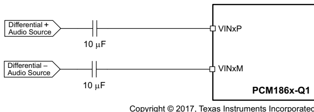
Figure 62. Analog Input Circuit for Differential Input Applications
