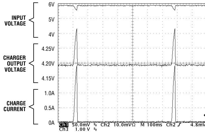
Figure 3. Overcurrent Protection
