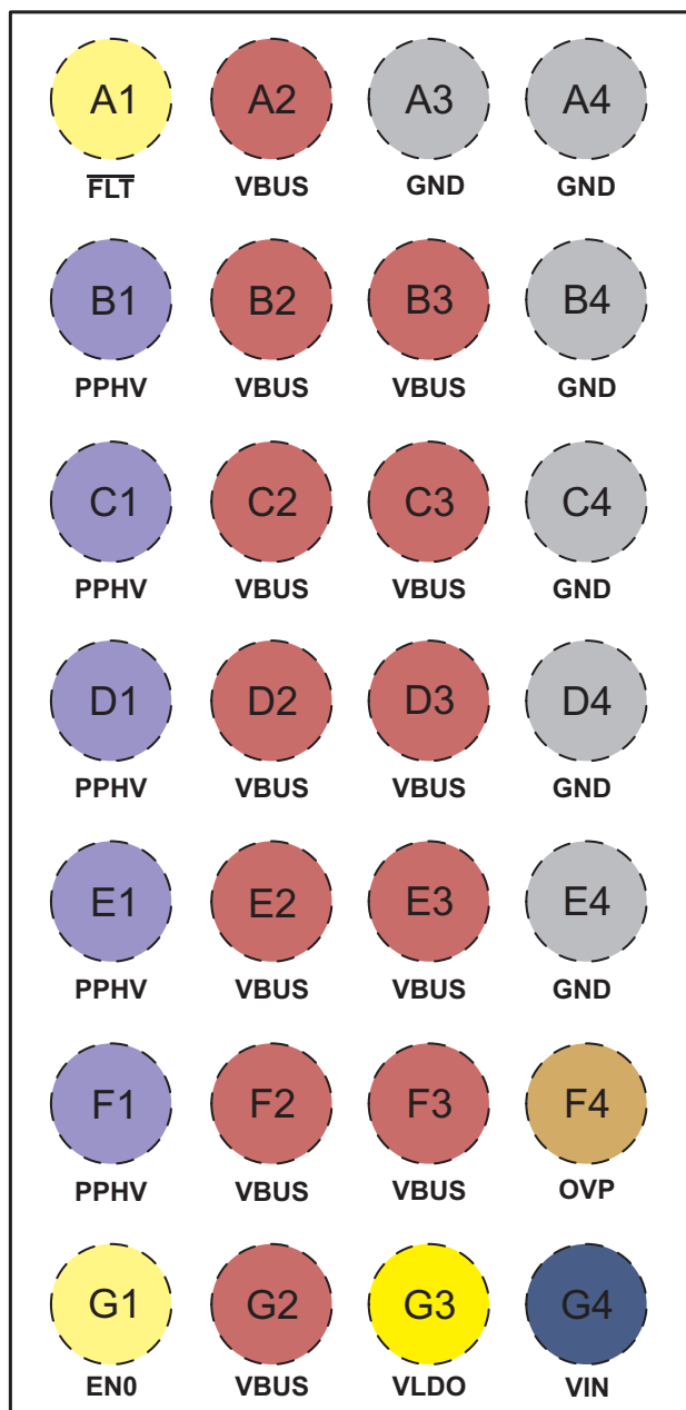
TPS6612x YBG Package 28-Pin WCSP Top View
