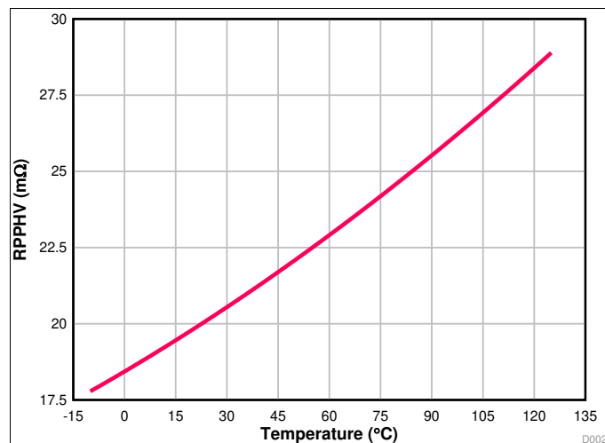
Figure 1. R_{PPHV} versus Temperature
