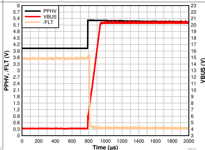
Figure 4. V_{BUS} OVP Response with 6-V Threshold
