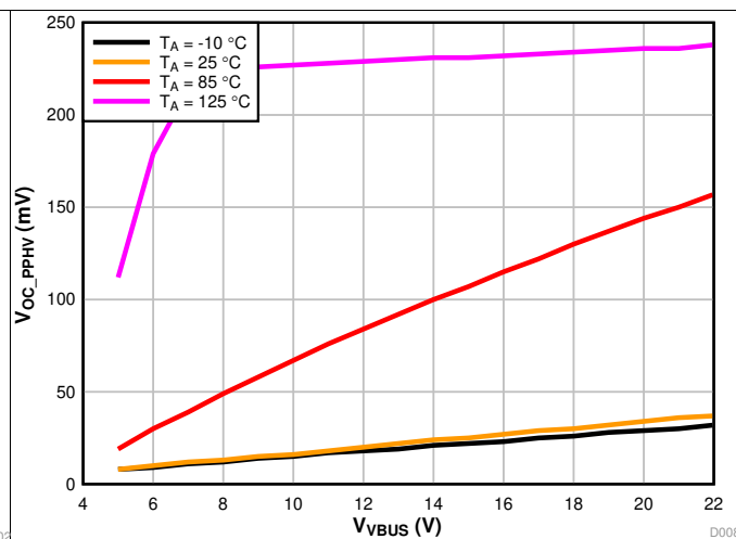
Figure 2. V_{OC\_PPHV} , PPHV Open Circuit Voltage versus V_{BUS}
