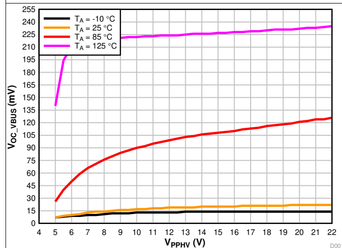
Figure 3. V_{OC\_VBUS} , V_{BUS} Open Circuit Voltage versus PPHV
