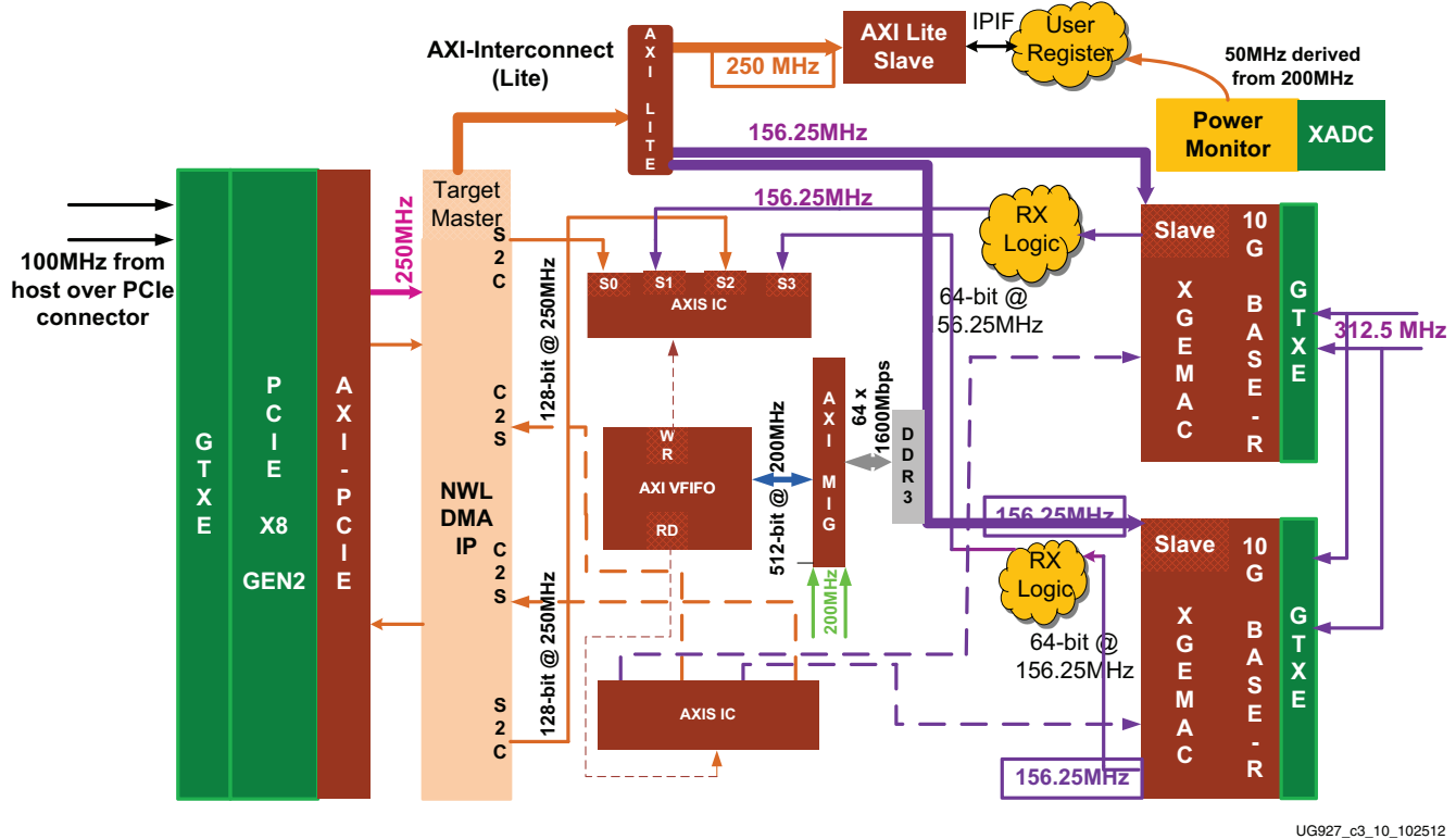
Figure 3-9: Clocking Scheme
