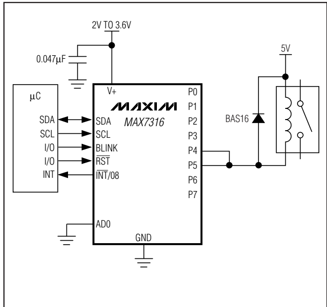
Figure 19. Diode-Protected Switching Inductive Load
