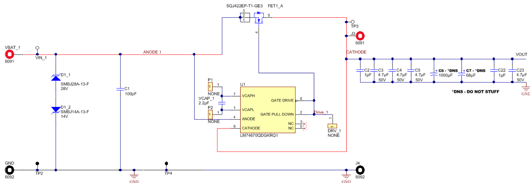
Figure 9. LM74670-Q1-SQEV Schematic
