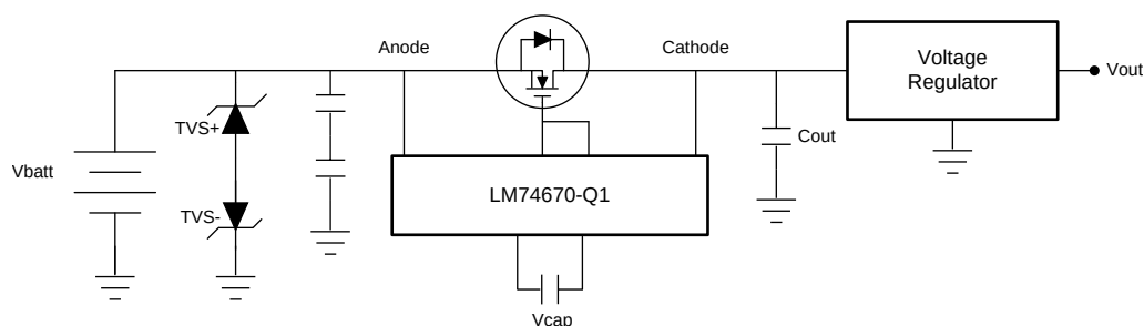
Figure 1. LM74670-Q1 Typical Application Circuit
