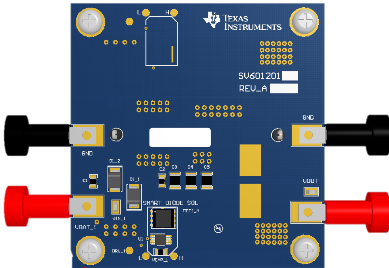
Figure 2. LM74670-Q1-SQ EVM
