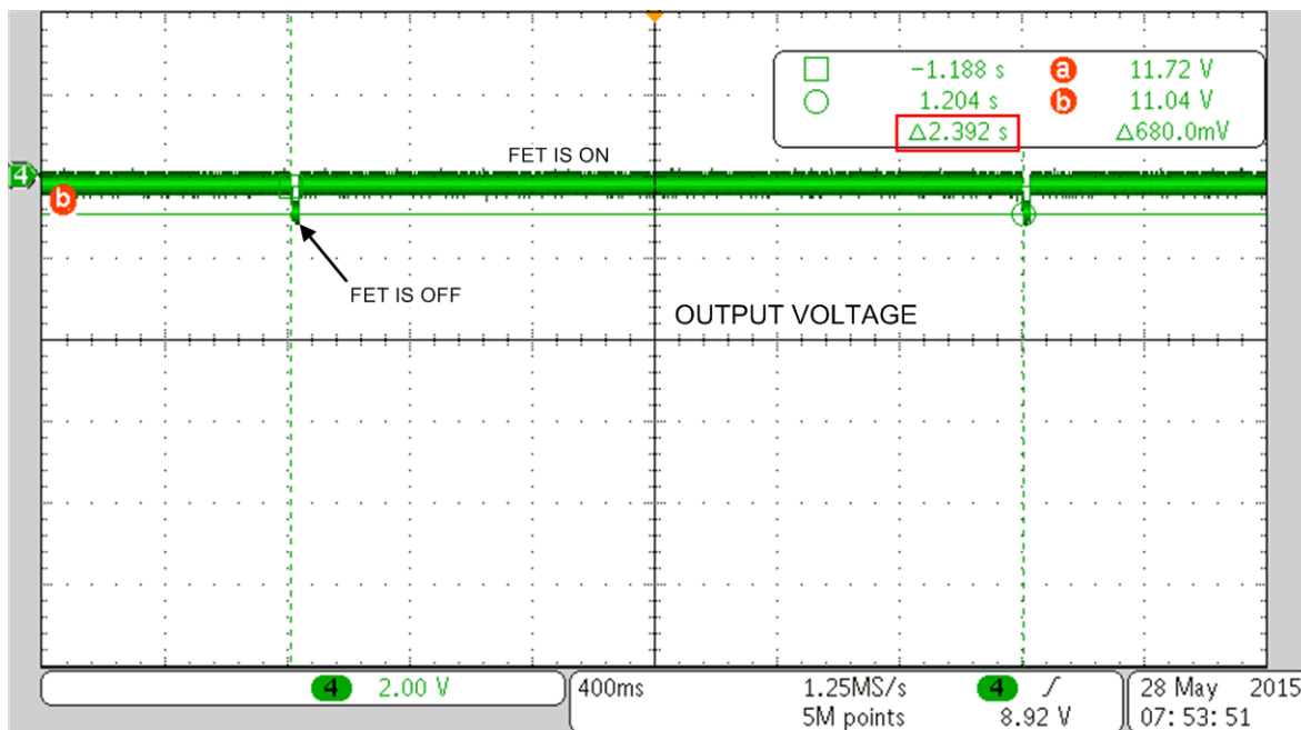
Figure 6. The LM74670-Q1-SQEVm Output voltage waveform
