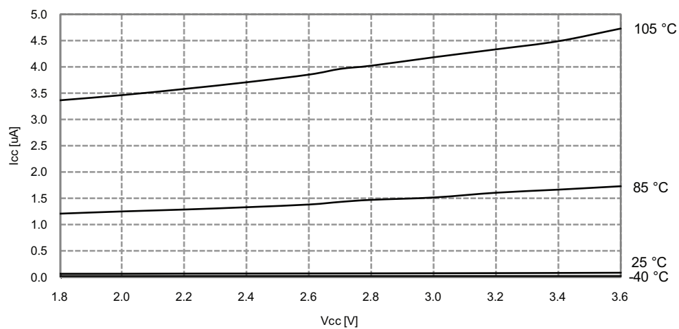
Figure 33-258. Power-down Mode Supply Current vs. V_{CC} All functions disabled
