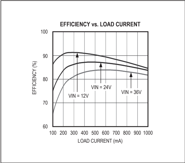
Figure 2. MAX17502E Efficiency
