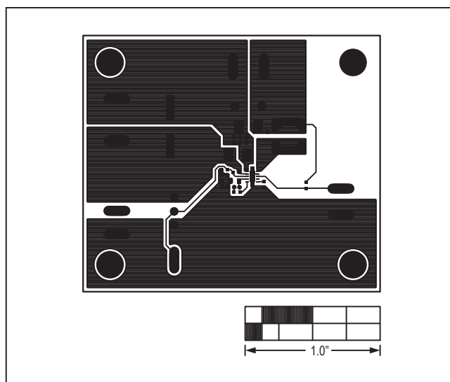
MAX17502E EV Kit PCB Layout—Component Side
