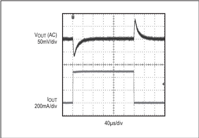
Figure 4. MAX17502E No Load to 500mA Load Transient
