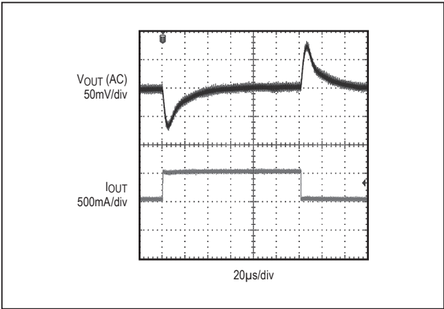
Figure 5. MAX17502E 500mA to 1A Load Transient
