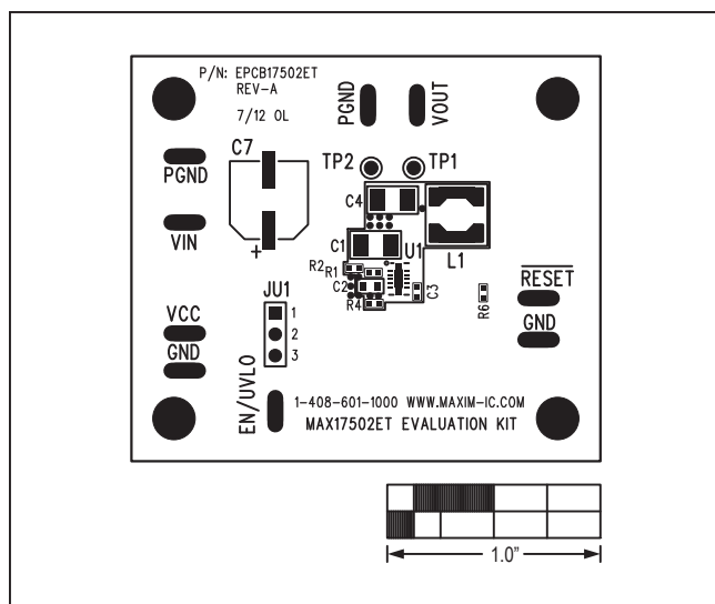
MAX17502E EV Kit Component Placement Guide— Component Side
