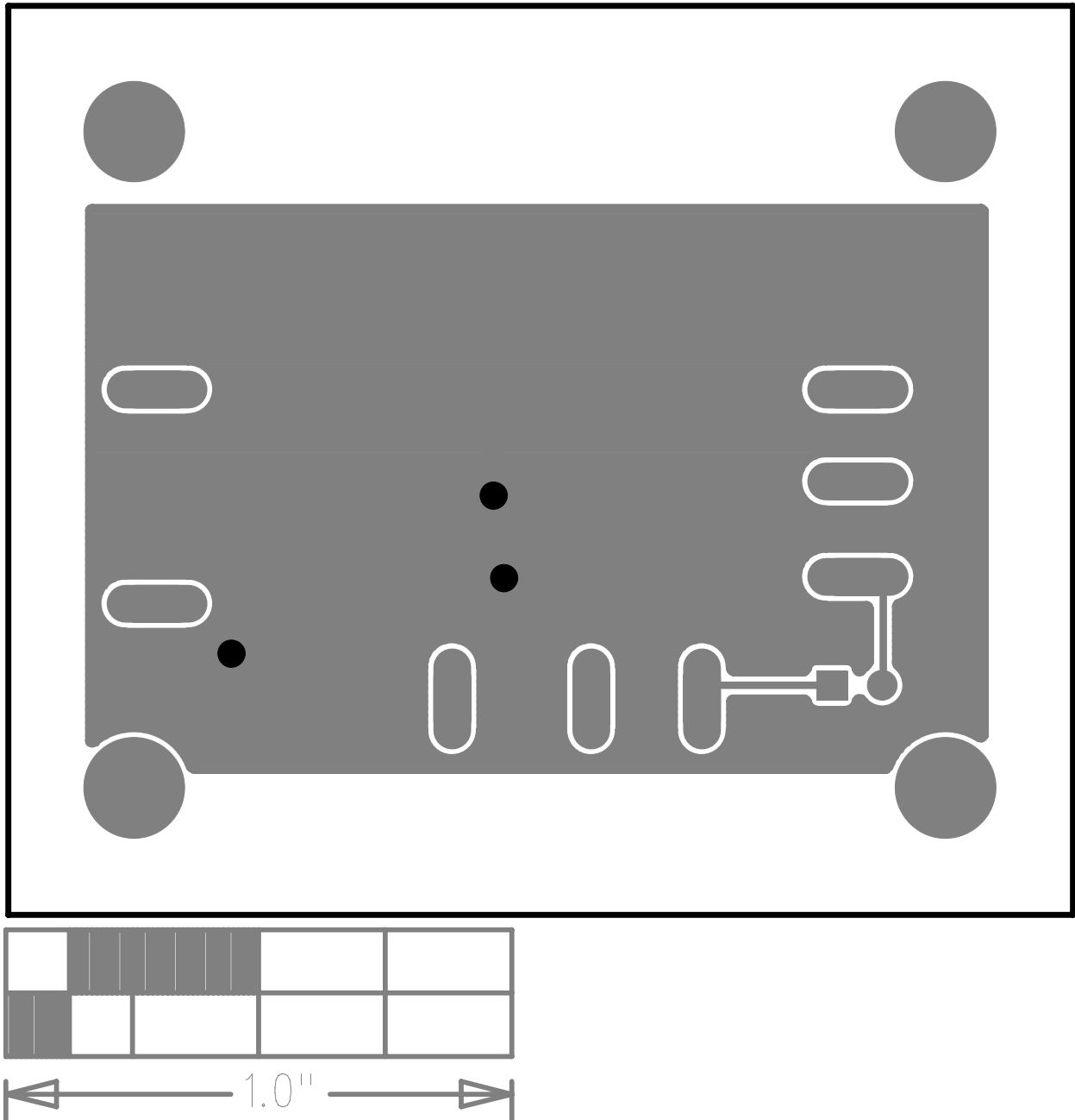
Figure 5. MAX8814 EV Kit PCB Layout—Solder Side
