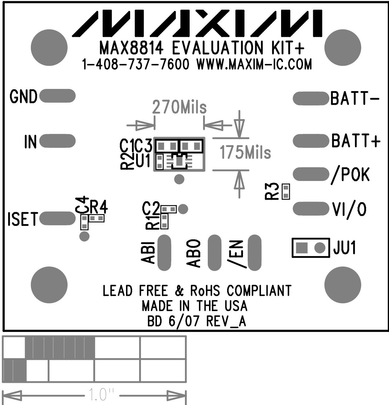
Figure 3. MAX8814 EV Kit Component Placement Guide—Component Side
