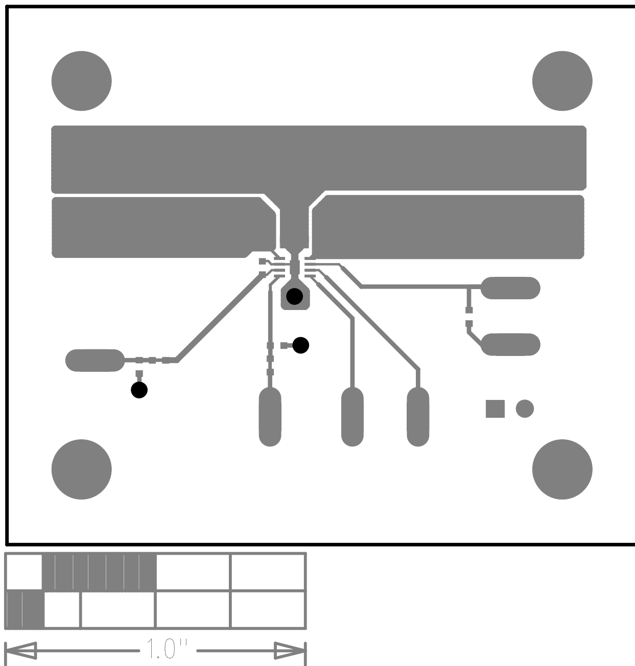
Figure 4. MAX8814 EV Kit PCB Layout—Component Side
