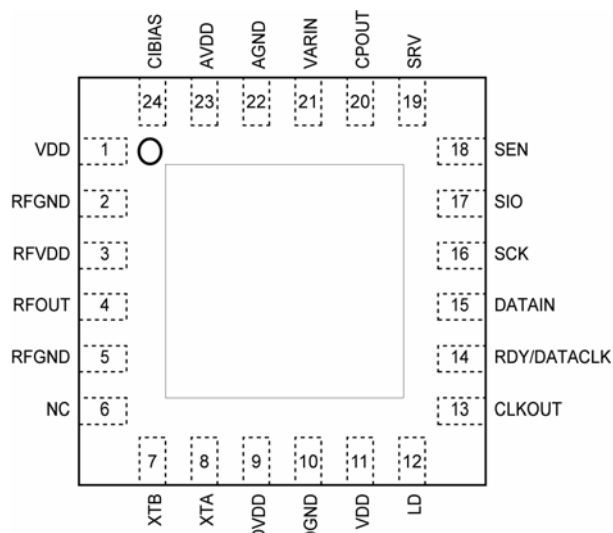
24-Pin MLC® (Top View)
