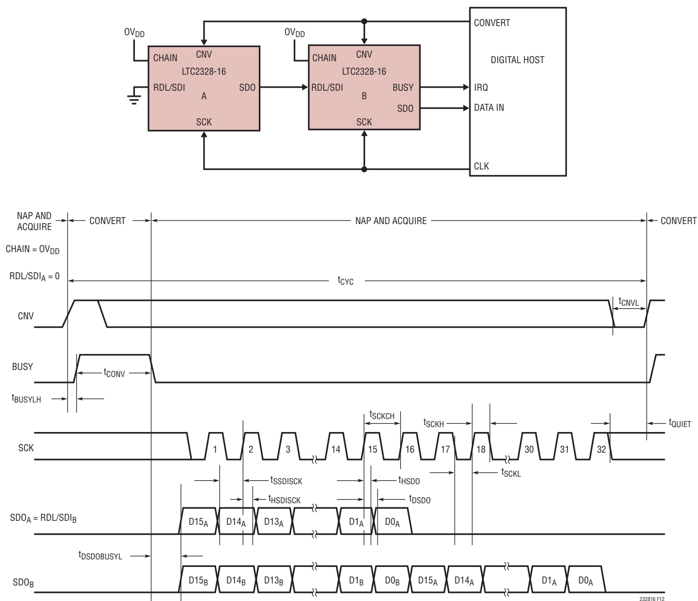
Figure 12. Chain Mode Timing Diagram
