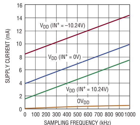
Supply Current vs Sampling Rate
