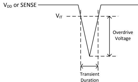
Figure 14. Overdrive Voltage
