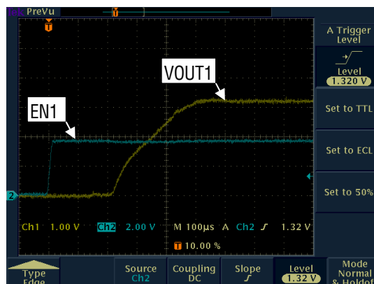
Figure 1. VOUT1 startup
