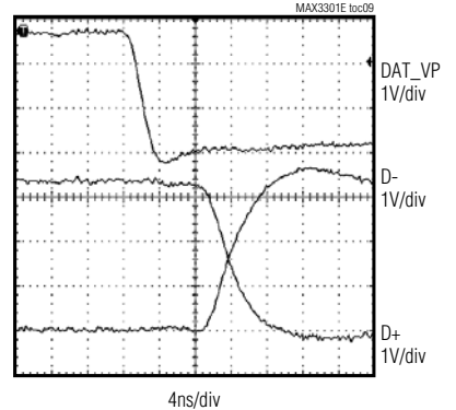
DRIVER PROPAGATION DELAY HIGH-TO-LOW (FULL-SPEED MODE)
