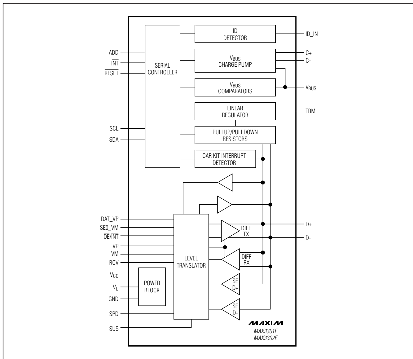
Figure 11. Block Diagram
