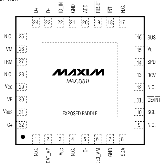
TQFN (5mm x 5mm)
