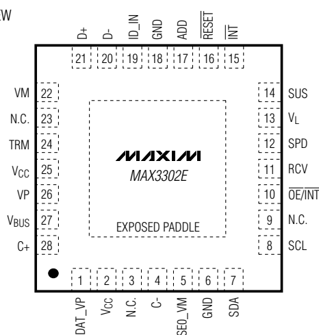
TQFN (4mm x 4mm)
