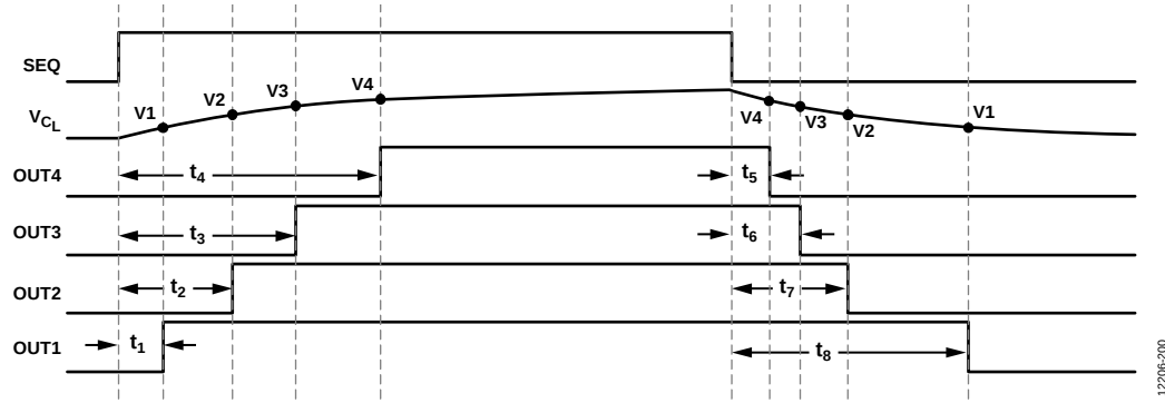
Figure 28. Mirrored Voltage Sequencer Timing Diagram
