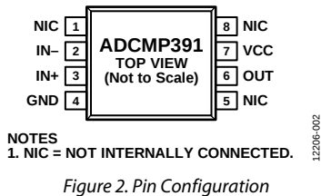
Figure 2. Pin Configuration
