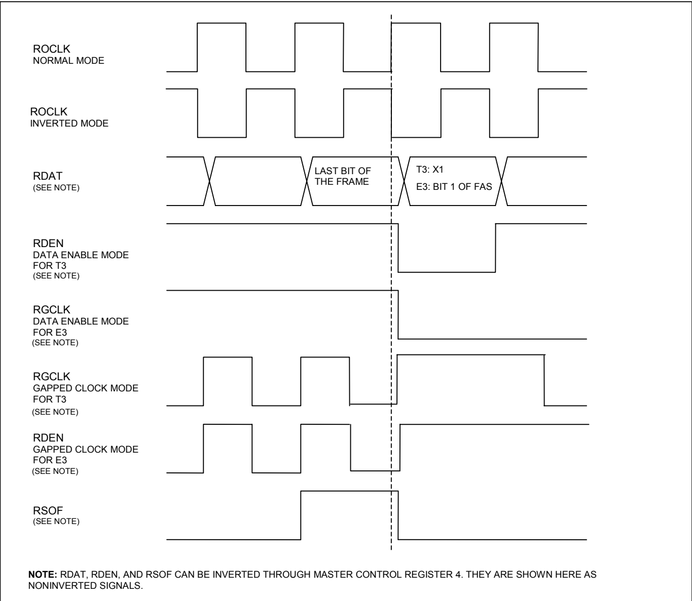
Figure 5-2. Receive Framing Timing
