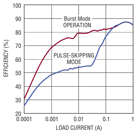
Figure 3. VOUT1 Measured Efficiency at V_{IN} = 12V , V_{OUT1} = 2.5V , L1 = 3.3\mu H , f_{SW} = 1MHz (with VOUT2 OFF)
