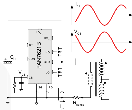
Figure 26. Full-Wave Sensing
