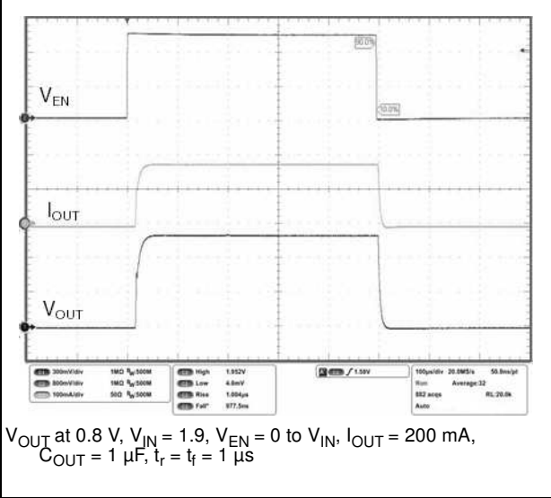
Figure 31. Enable transient ( V_{OUT} = V_{ADJ} )
