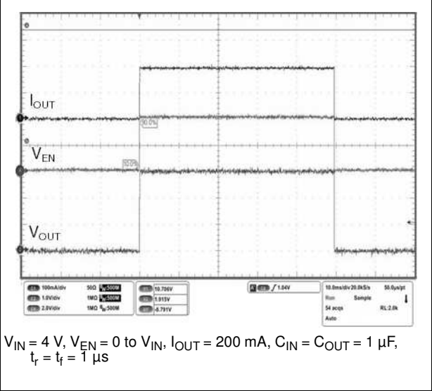
Figure 32. Enable transient ( V_{OUT} = 3 V)
