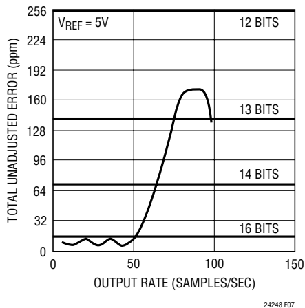
Figure 7. Total Error vs Output Rate ( V_{BFF} = 5V )
