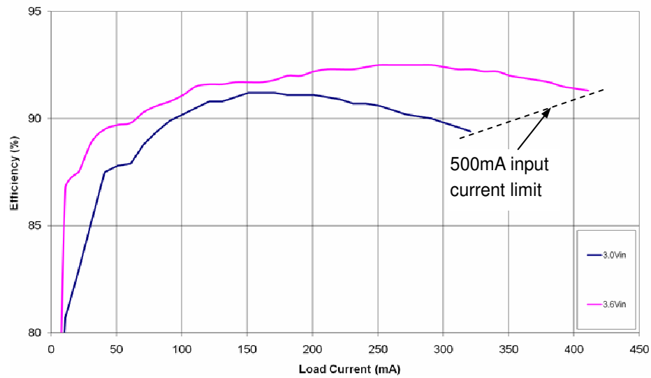
Figure 4. Typical Efficiency vs. Load Current
