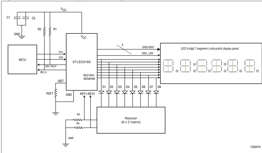
Figure 9. STLED316S application diagram
