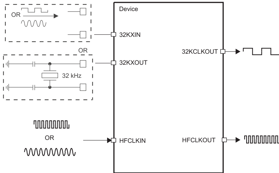
Figure 5-61. Clock Overview
