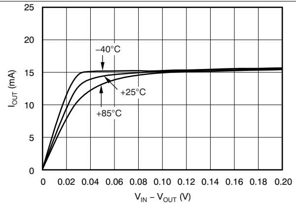
Figure 6. Output Current vs Headroom Voltage
