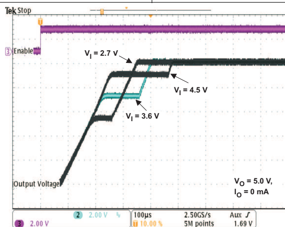
Figure 37. Start-Up
