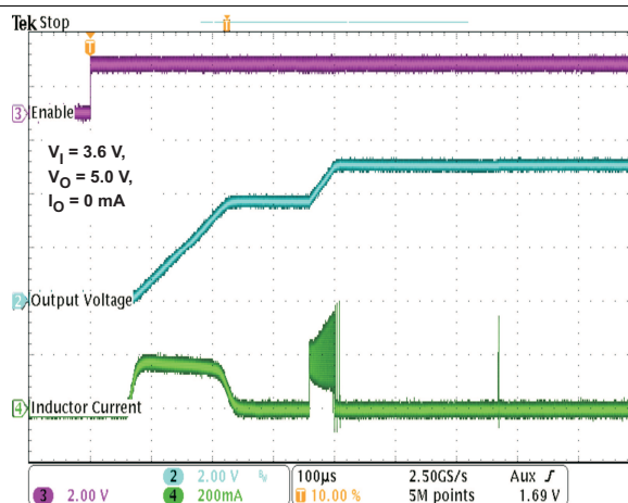
Figure 36. Start-Up
