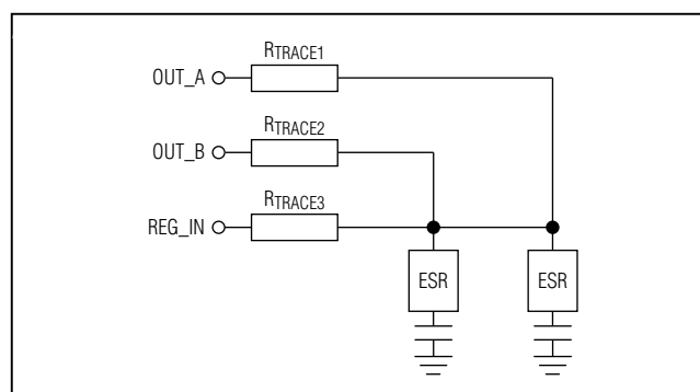
Figure 19. Output Capacitor Star Connection
