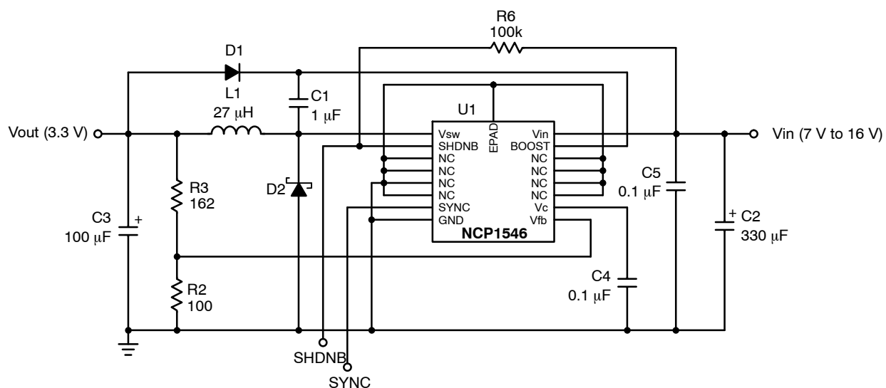
Figure 1. Application Diagram, 4.5 V – 16 V to 3.3 V @ 1.0 A Converter
