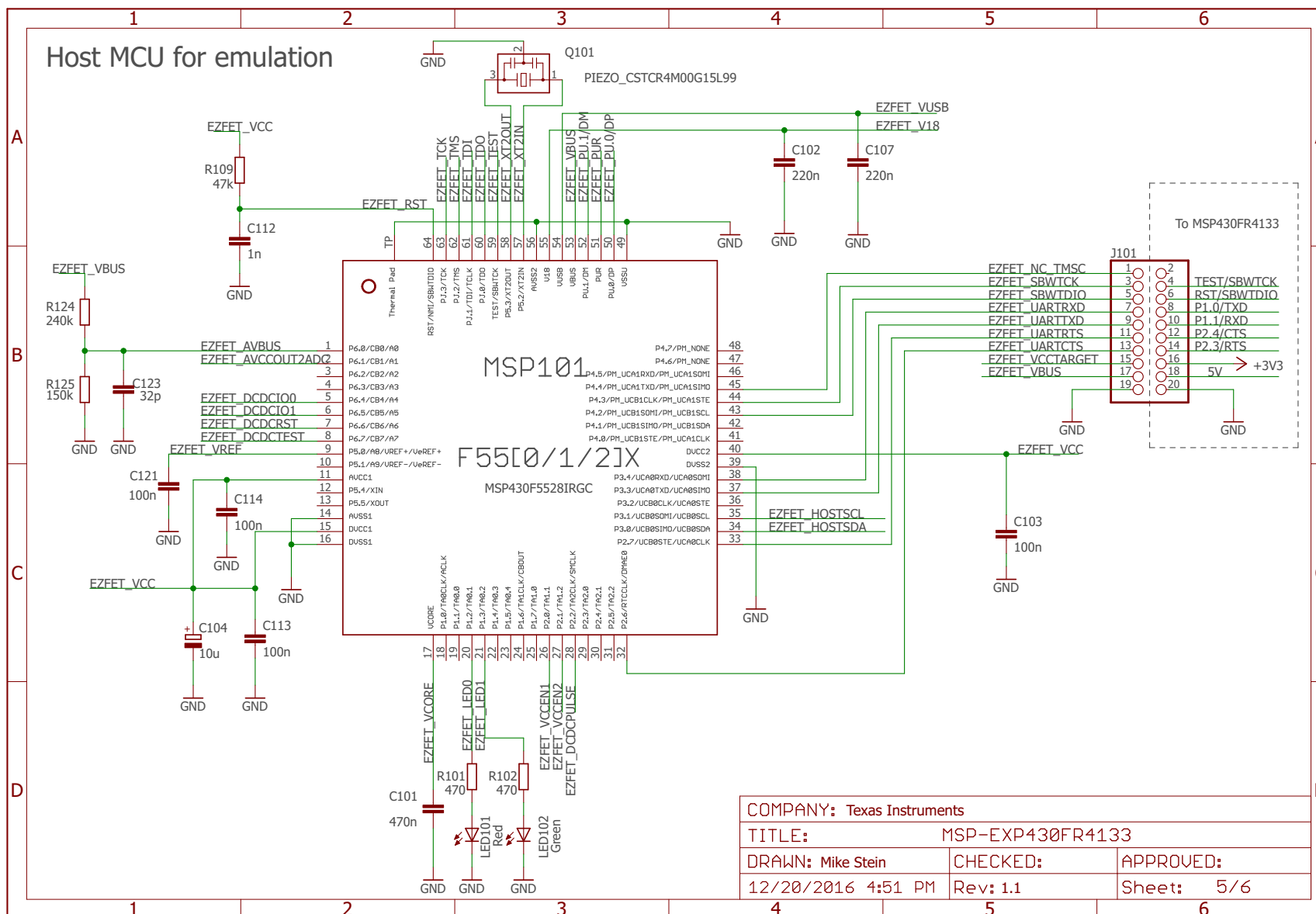
Figure 19. Schematics (5 of 6)
