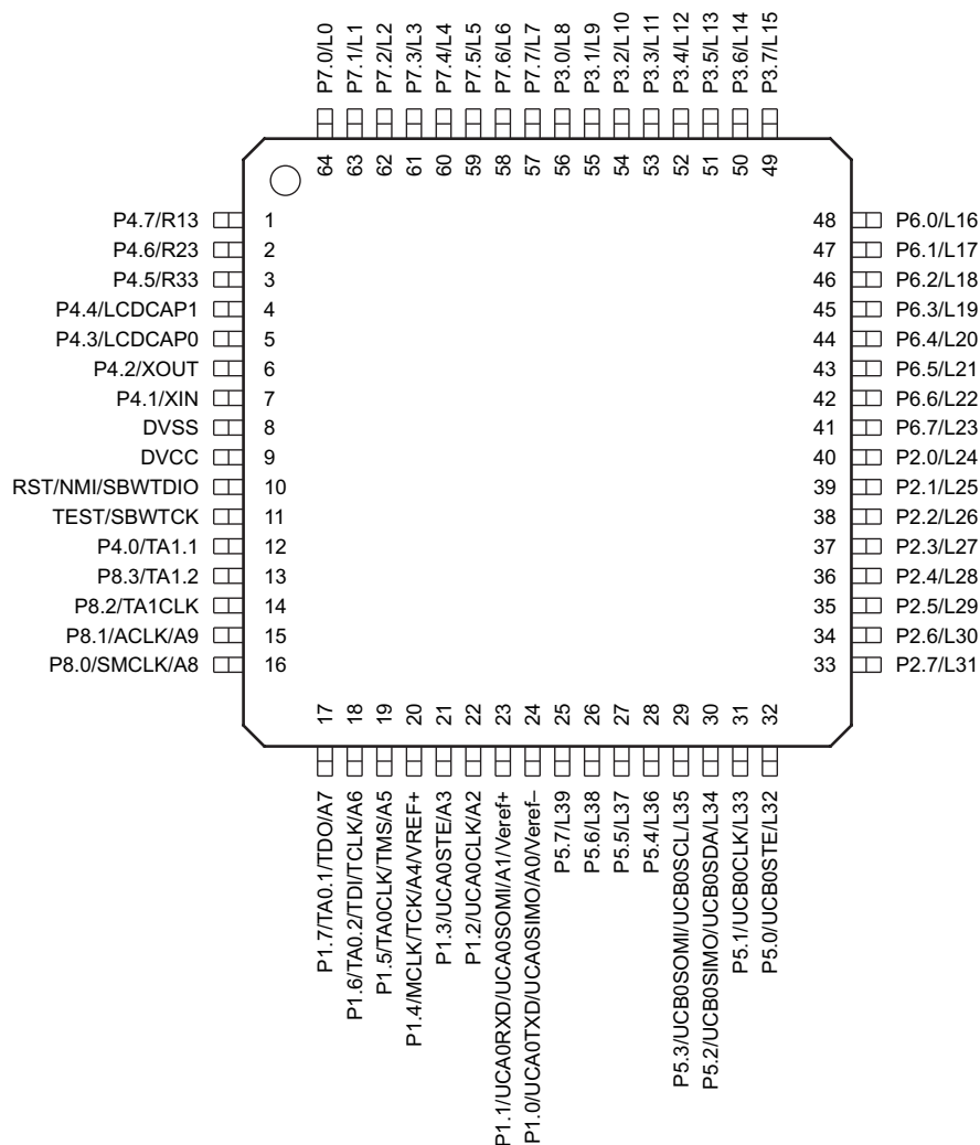
Figure 4. MSP430FR4133 Pinout
