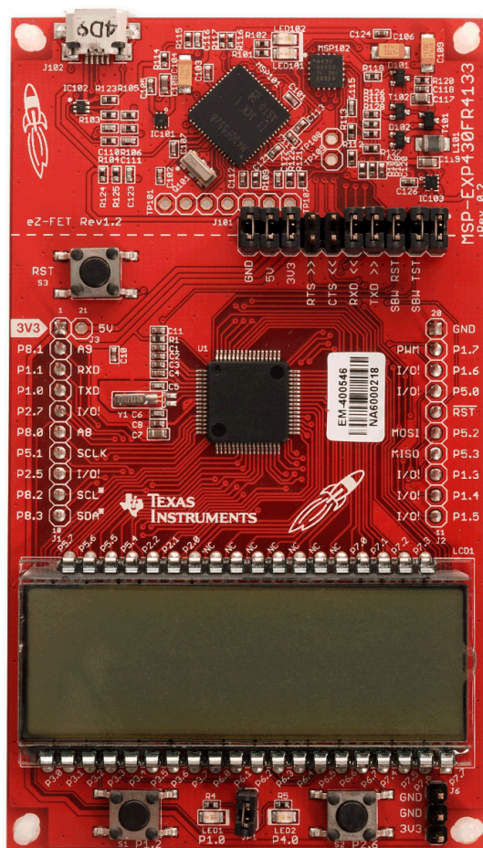
Figure 1. MSP-EXP430FR4133
