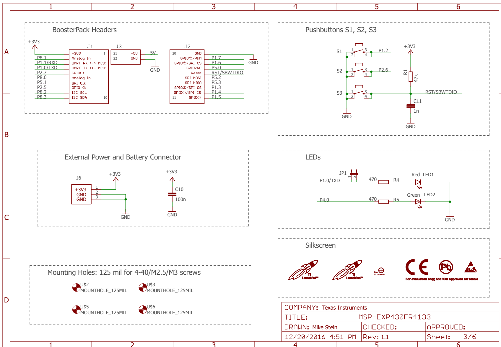
Figure 17. Schematics (3 of 6)
