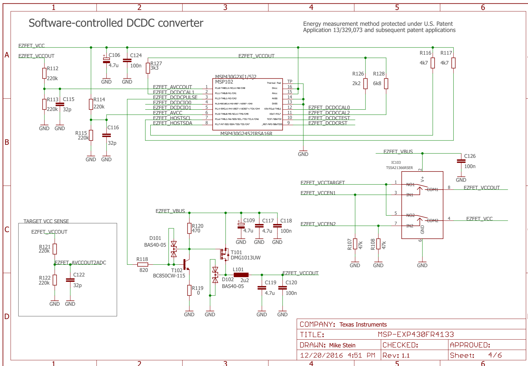
Figure 18. Schematics (4 of 6)
