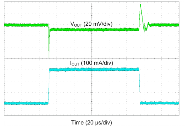
Figure 51. LDO Transient Load Step Response
