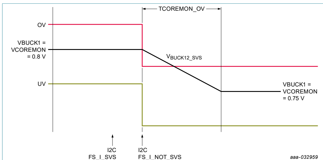
Figure 41. SVS principle
