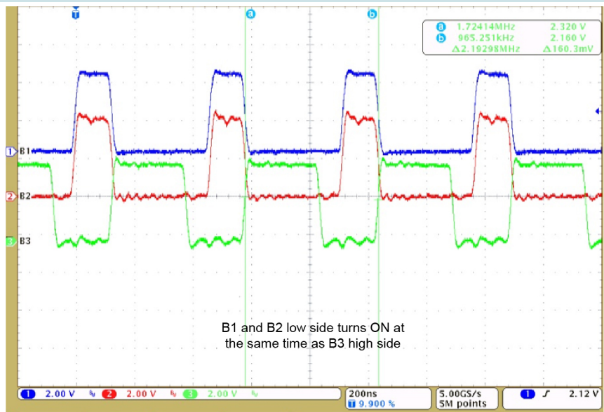
Figure 30. BUCK1,2,3_clk = 2.22 MHz without clock phase shifting
