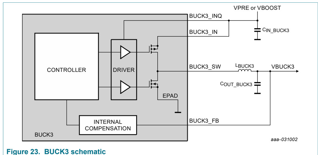
Figure 23. BUCK3 schematic
