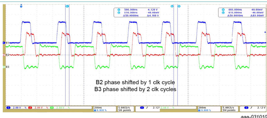
Figure 31. BUCK1,2,3_clk = 2.22 MHz with clock phase shifting
