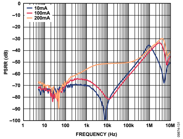
Figure 31. Power Supply Rejection Ratio vs. Frequency, V_{OUT} = 3.3 V , V_{IN} = 3.8 V , V_{RIPPLE} = 50 mV , C_{OUT} = 1 \mu F
