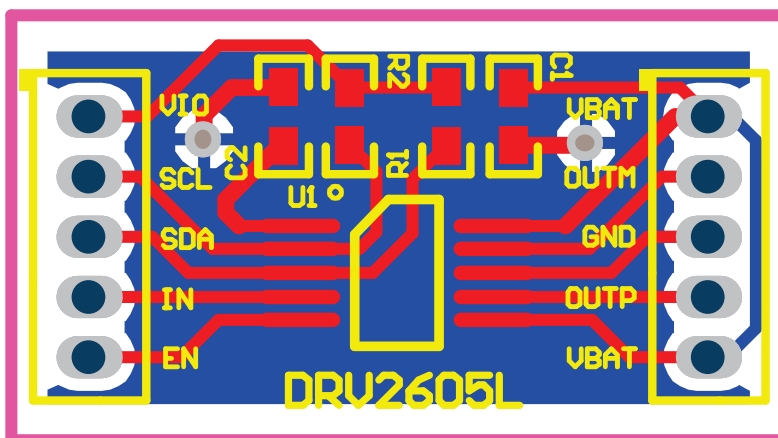
Figure 5. Top Silkscreen (Yellow), Top (Red), and Bottom (Blue) Layers
