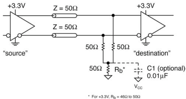
Figure 3. Three-Resistor "Y-Termination"
