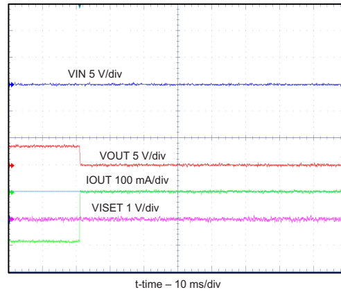
Figure 12. Battery Removal
