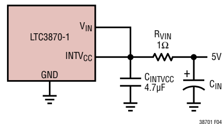
Figure 2. Setup for a 5V Input
