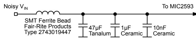
Figure 14. Filter Circuit for Noisy Supplies ( +3.3\text{V} and/or -12\text{V} )
