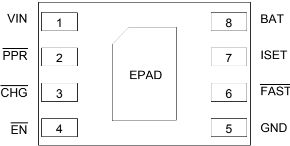
Figure 3. 34671 Pin Connections
