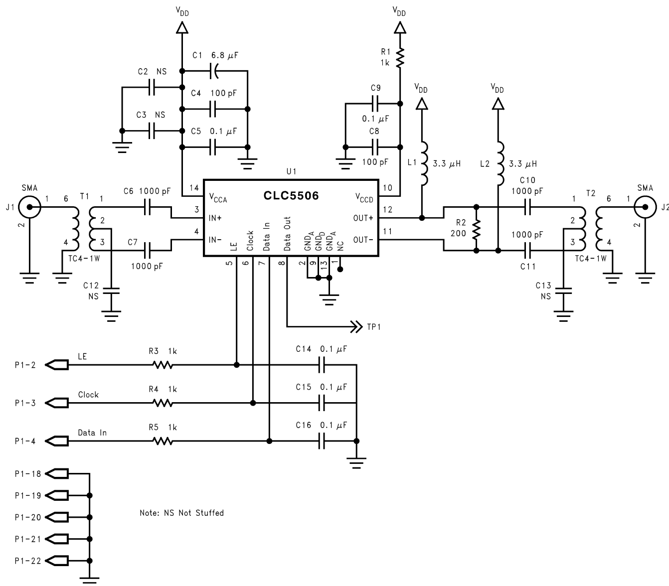
Figure 1. CLC5506PCASM Schematic Diagram
