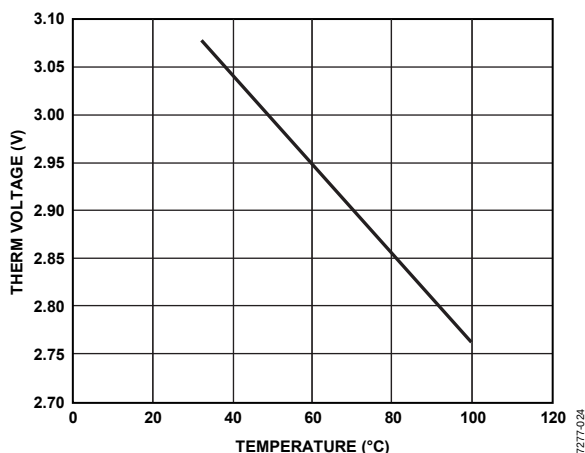
Figure 24. Temperature Sensor Output Voltage vs. Temperature
