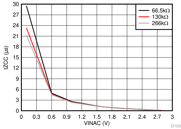
Figure 1. RTSET Resistance and Zero-Crossing Distortion Correction Additional On Time
