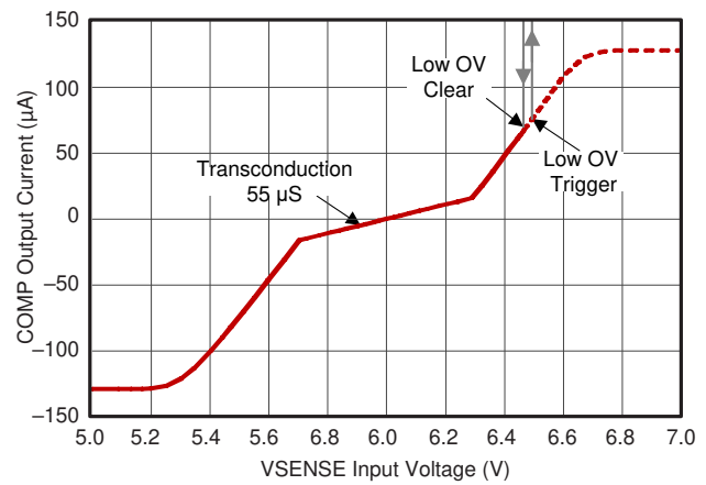
Figure 8. Error Amplifier Output Current vs Input Voltage
