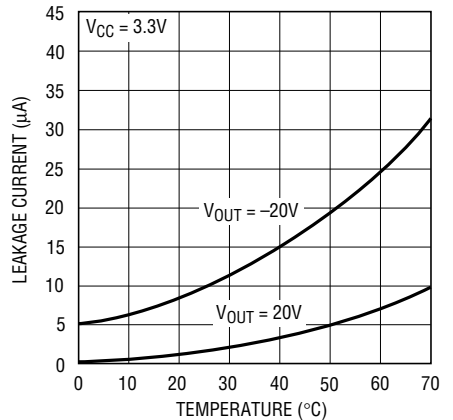
Driver Leakage in SHUTDOWN vs Temperature ( ^{\circ}\text{C} )
