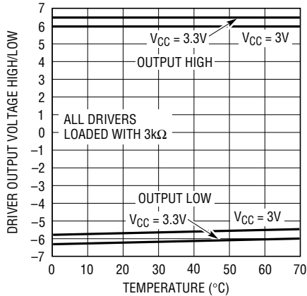
Driver Output Voltage High/Low vs Temperature ( ^{\circ}\text{C} )
