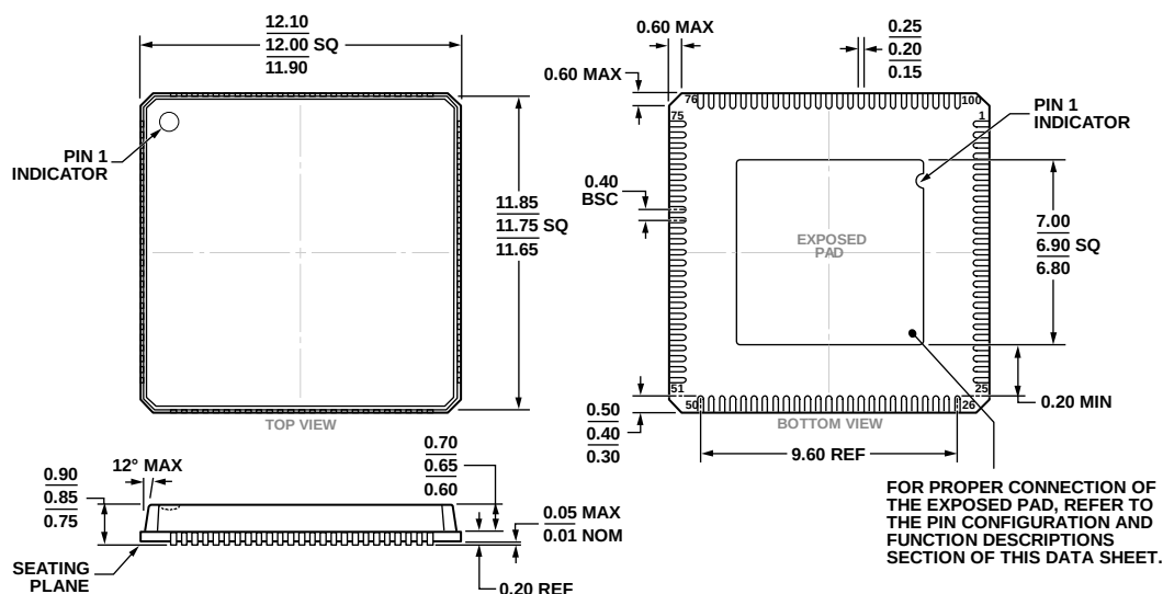
Figure 66. 100-Lead Lead Frame Chip Scale Package [LFCSP_VQ]
