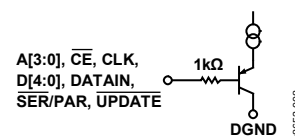
Figure 61. Logic Input
