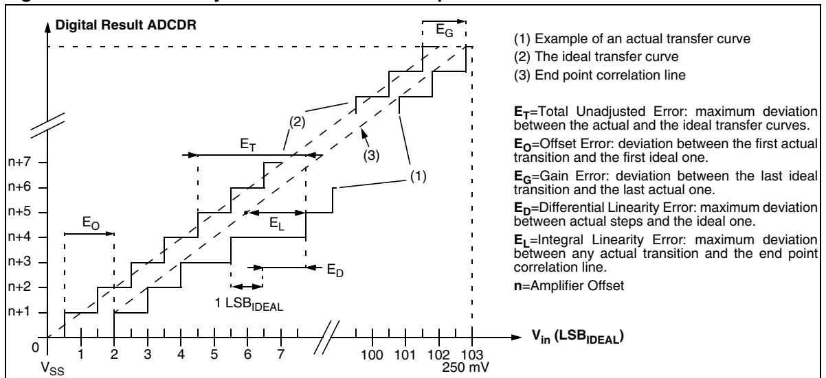
Figure 85. ADC Accuracy Characteristics with Amplifier enabled
