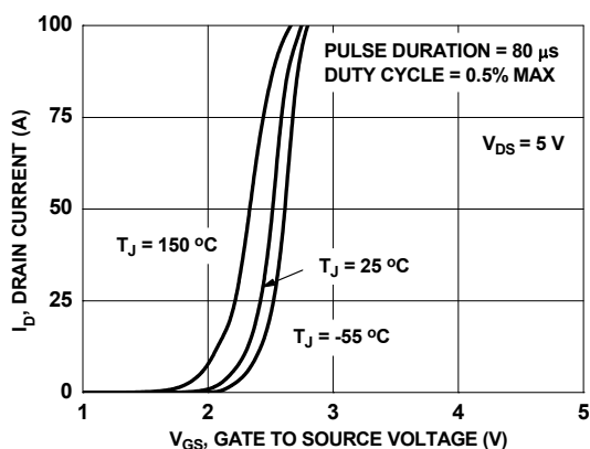
Figure 20. Transfer Characteristics
