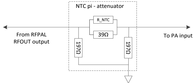
Figure 5: NTC Attenuator
