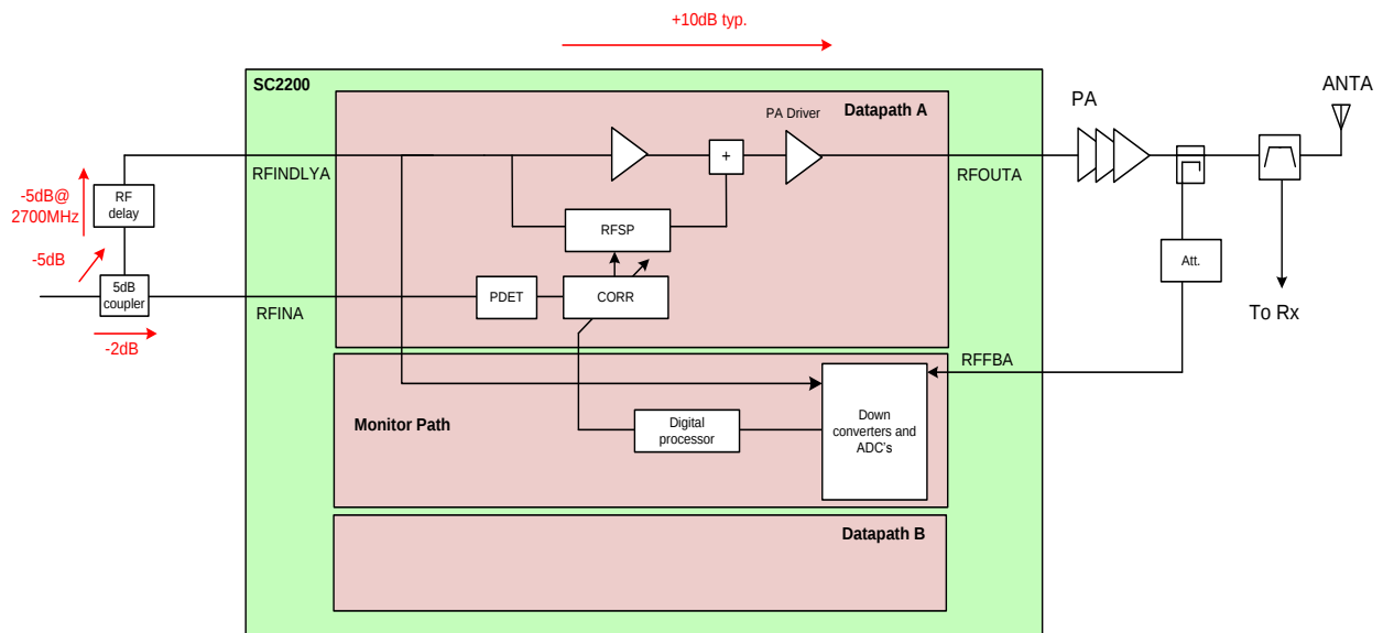
Figure 4: SC2200 with Delay Line RF Circuit Block Diagram
