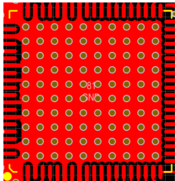
Figure 11: Via Array Under SC2200 Ground Paddle
