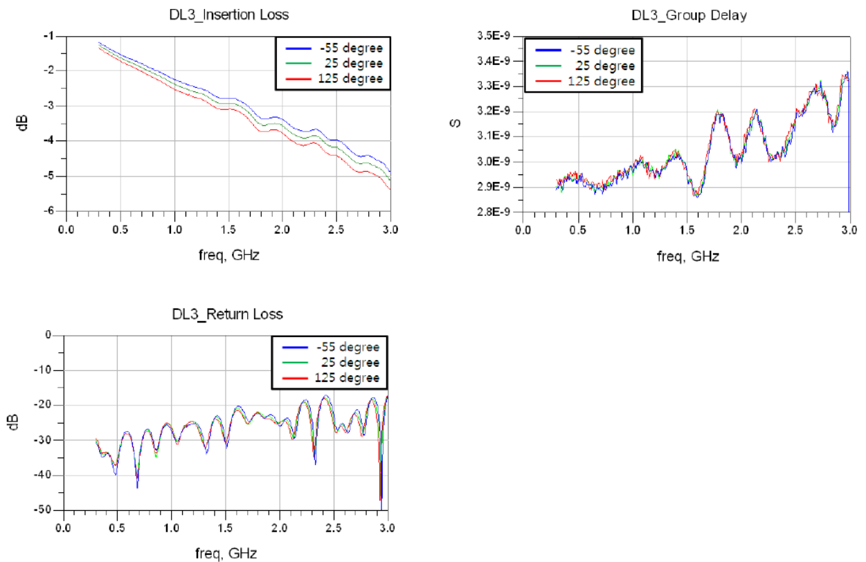
Figure 7: DL3 Delay Line Insertion Loss (dB), Delay (s) and Return Loss (dB)
