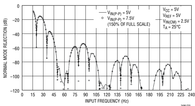
Figure 20. Input Normal Mode Rejection vs Input Frequency with Input Perturbation of 150% (60Hz/60Hz Notch)
