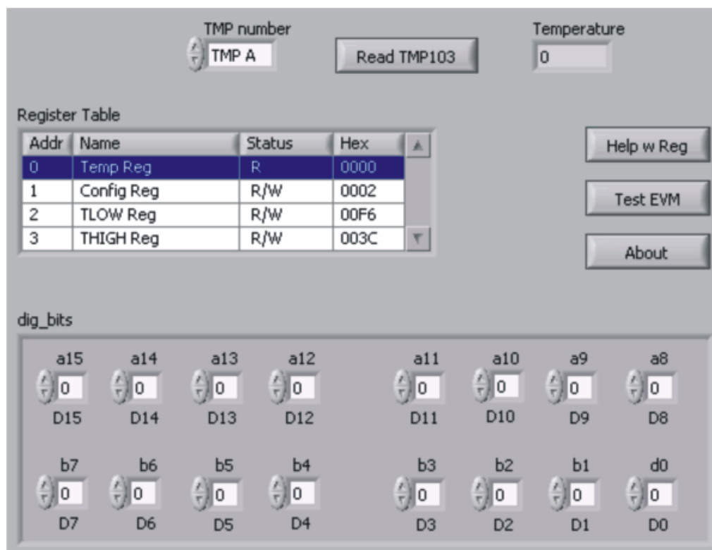
Figure 20. TMP103EVM Software: Register Tab
