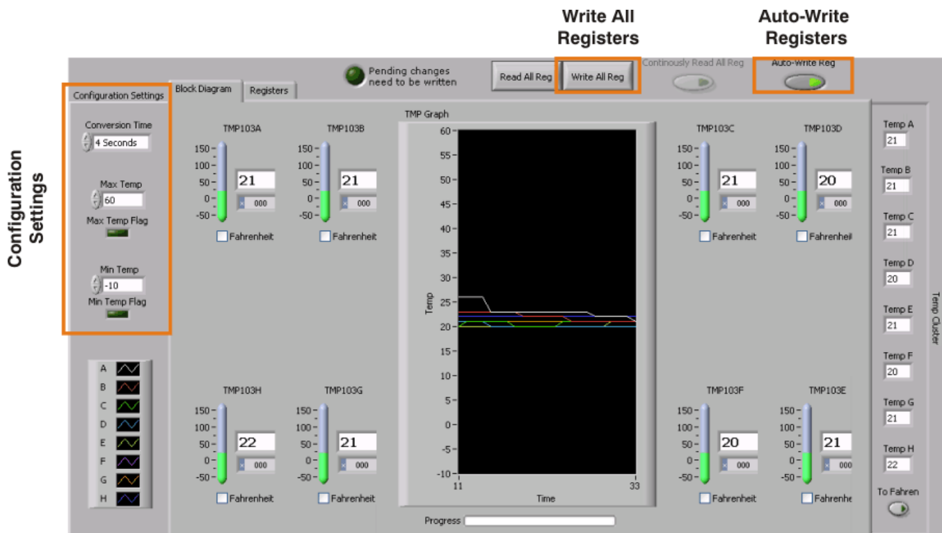
Figure 17. TMP103EVM Software: Writing to Registers
