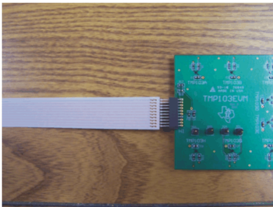
Figure 7. 10-Pin Ribbon Cable Extender
