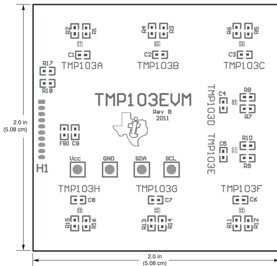
Figure 23. TMP103EVM Component Layout
